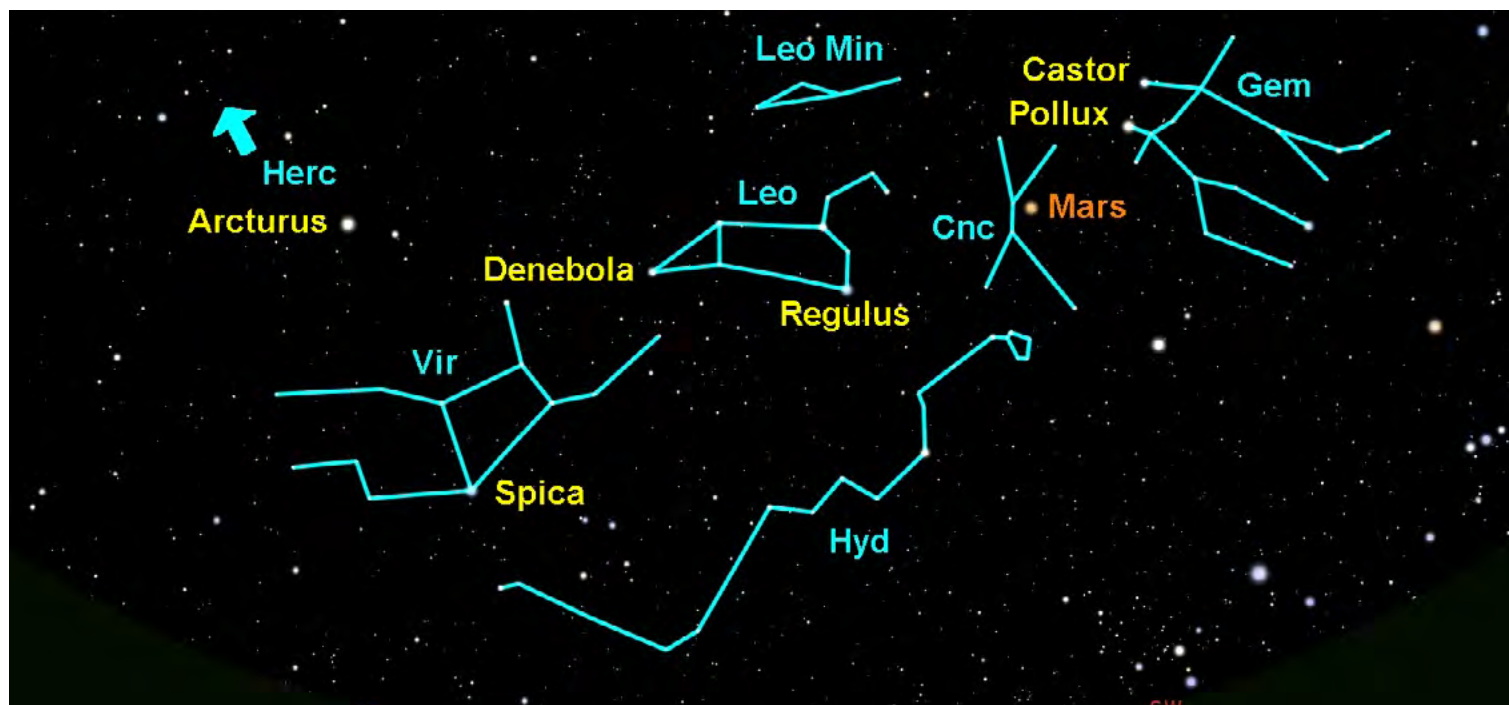
A view to the south at 9:30 pm on May 1. From Stellarium .
